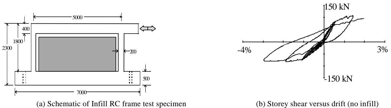
Figure 4. Test results for 1/2-scale r/c frame subject to cyclic loading (Griffith and Alaia, 1997).
