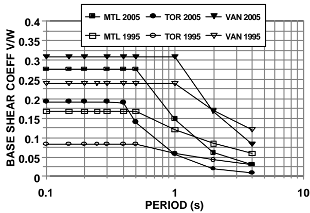
Figure 3 Conventional Construction Steel Moment Frame on Soft Soil
