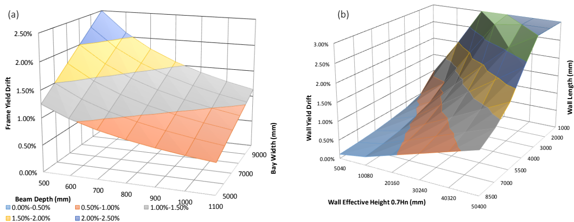
Figure 3: (a) RC moment-frame nominal yield drift as a function of beam-bay span and depth (b) RC shear-wall nominal yield drift as a function of wall effective height ( 0.7H_n ) and wall length. First yield is assumed to typically occur at 65-75% of nominal yield.
