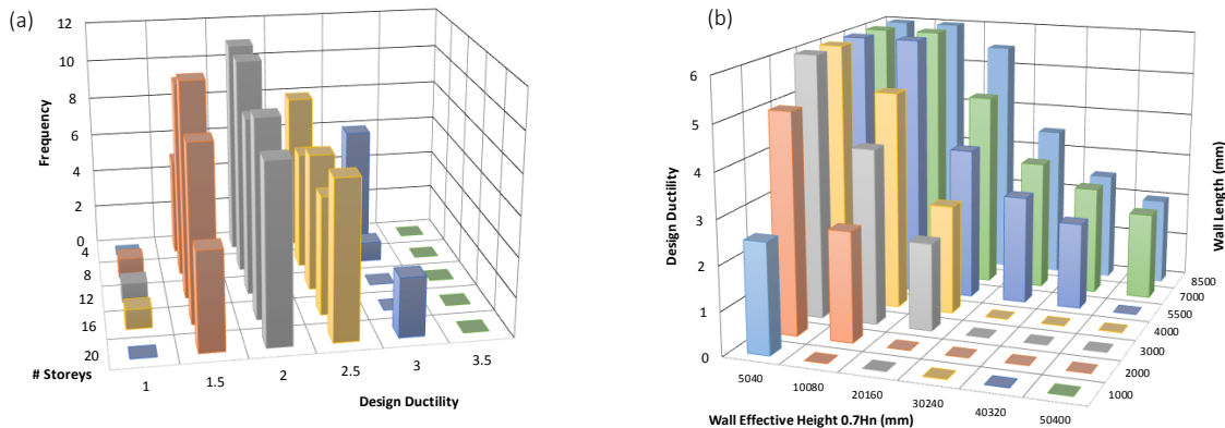
Figure 4: (a) RC moment-frame design ductility for the range of frame geometries in Figure 3a assuming peak storey drift is 2.5% (b) RC shear wall design ductility as a function of wall effective height ( 0.7H_n ) and wall length assuming peak storey drift of 2.5%.
