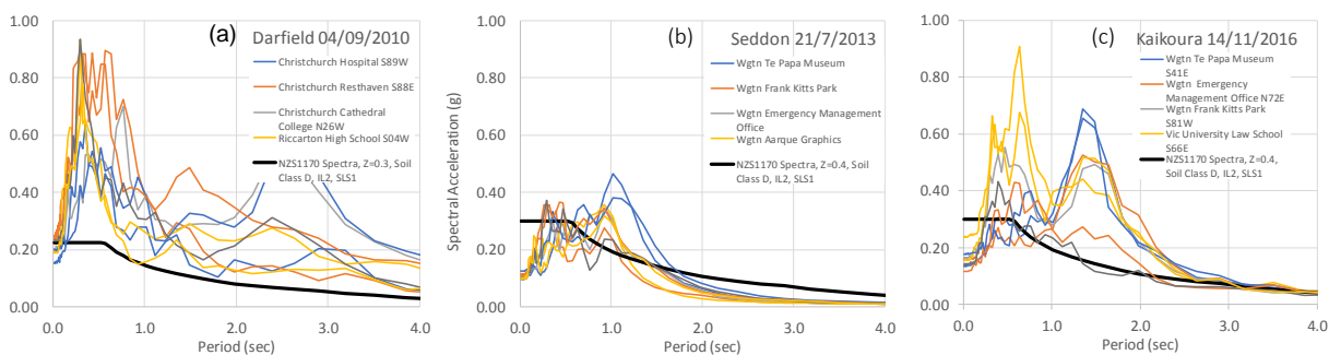
Figure 1: Acceleration spectra for (a) Darfield earthquake recorded in Christchurch (b) Cook Strait earthquake recorded in Wellington (c) Kaikoura earthquake recorded in Wellington.
