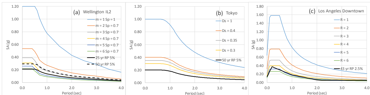
Figure 2: Comparison of design acceleration spectra for (a) Wellington ULS for range of ductility and with SLS1 25 year and 50 year spectra (b) Tokyo Level 2 for a range of RC frame D_s factors and Level 1 (c) Los Angeles DBE for a range of R -values and approximate SLE 43 year RP spectrum
