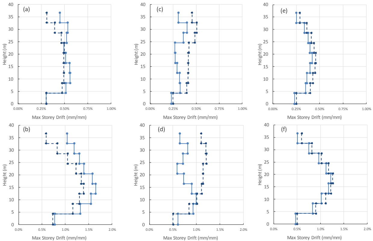
Figure 6: Average diaphragm centre-of-mass maximum storey drift profiles (a & b) Building 1 ULS design with \mu = 4 typical NZ design (c & d) Building 2 ULS design with \mu = 2 displacement-based ductility evaluated design (e & f) Building 3 SLS 50 year RP design with \mu = 2 displacement-based ductility evaluated design (e & f) Building 3 SLS 50 year RP design with \mu = 1 .
