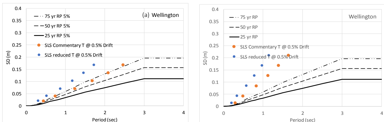
Figure 5: Centre-of-mass response building heights n = 2 to 20 . Orange dots represent design to typical ductility (likely \mu = 4 or more), blue dots represent the approximate the reduction of design ductility to 1.5 - 2.5 (a) RC frame approx. elastic period-design displacement points (b) RC shear wall approx. elastic period-design displacement. Allowance for torsion amplification of 20% has been made in determining a reduced centre-of-mass displacement.
