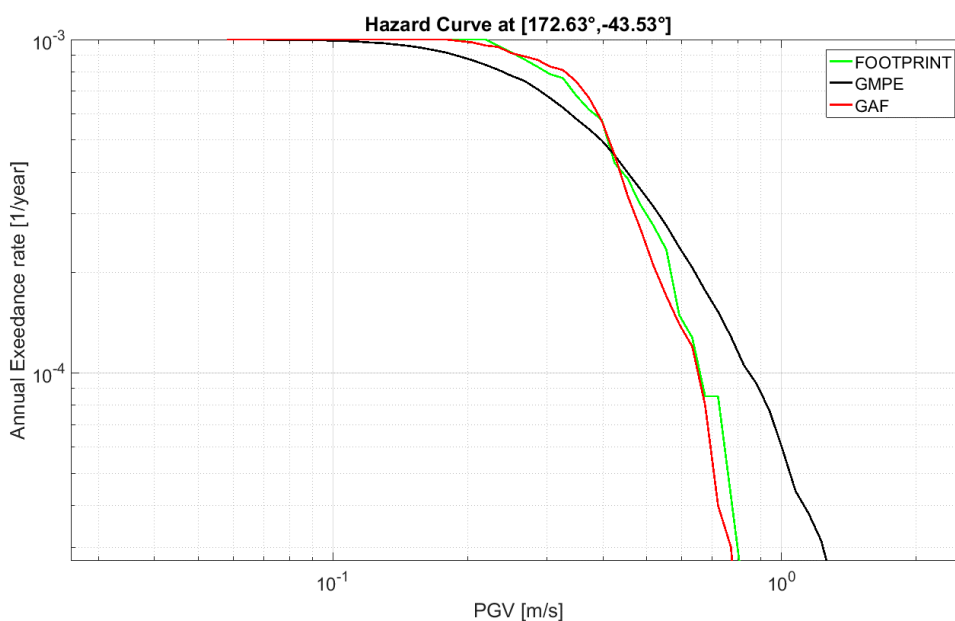
Figure 6: PGV Hazard Curve for the CBD in Christchurch (yellow point in Figure 5).
