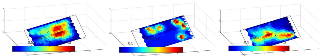
Figure 2: Example of three different slip pattern and hypocenter location for an hypothetical Mw 6.2 scenario generated on the “Christchurch” fault.
