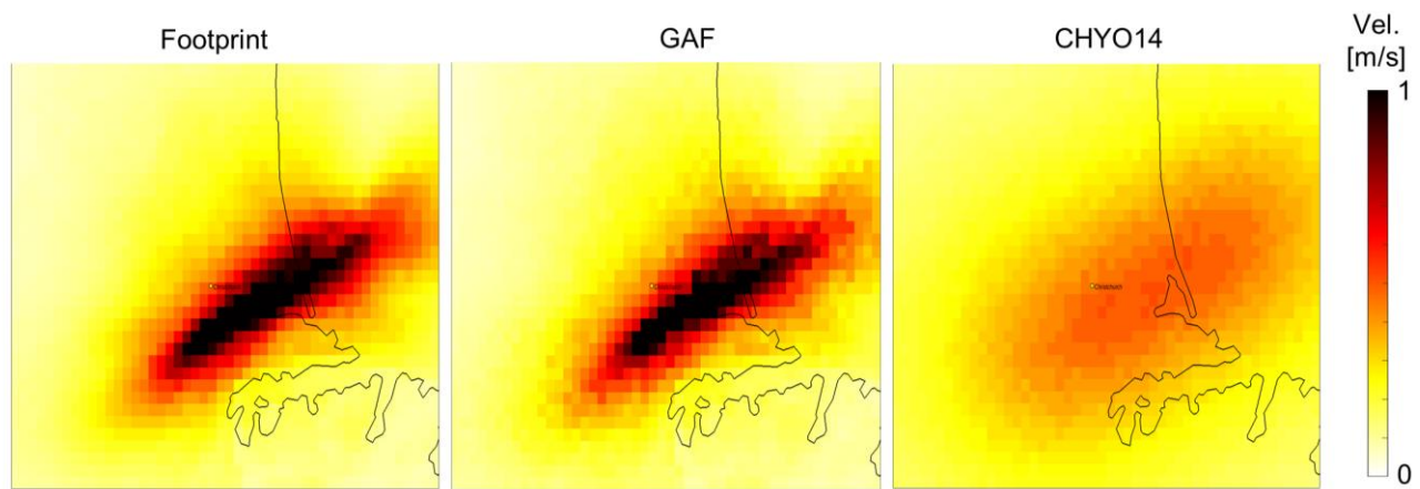
Figure 5: PGV Hazard Maps for T_r = 2475y obtained according to the Footprint (left), GAF (center) and GMM (right) method. The GMM used is the CHYO14.
