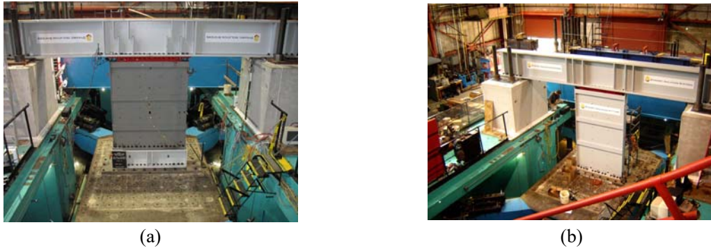
Figure 5: VWD full-scale testing: a) 7 ft \times 9 ft specimen, b) 7 ft \times 12 ft specimen
