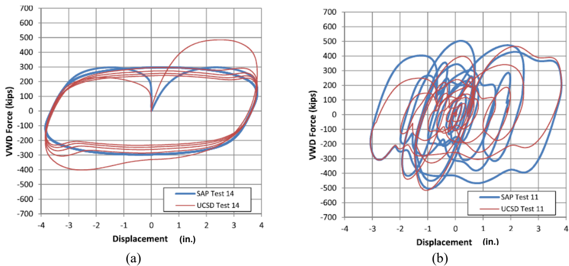
Figure 9: Force-displacement comparisons between UCSD test results and the analytical model for the 7ft \times 9ft VWD: a) Cyclic test with nominal properties and maximum velocity of 7.6 in/sec and b) Simulated earthquake test with \lambda_{test}=1.55 and maximum velocity of 11.3 in/sec
