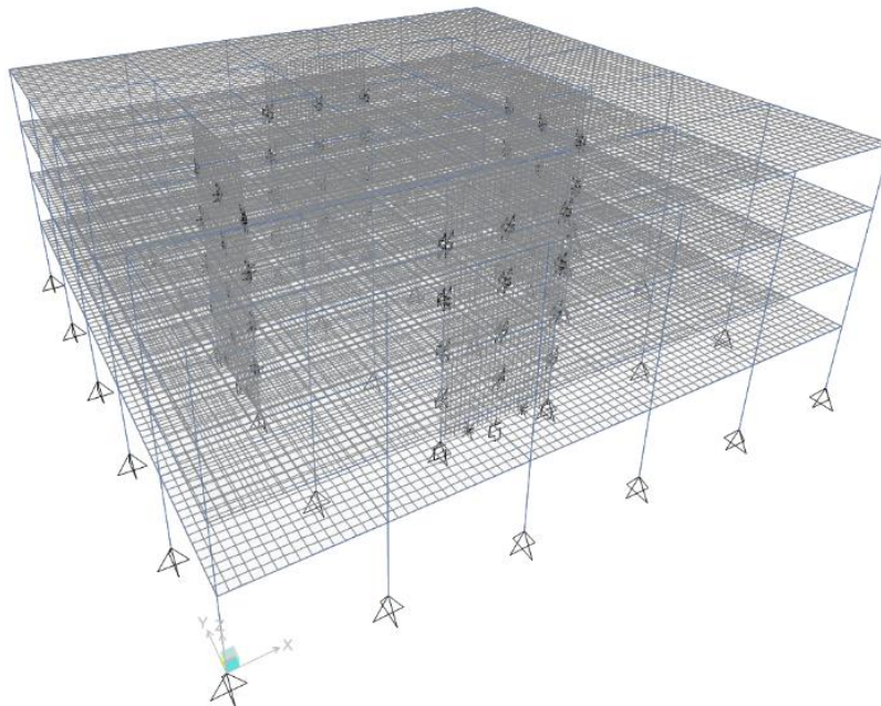
Figure 6. Numerical model of the prototype building
