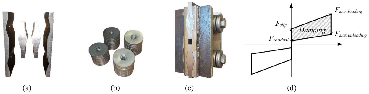
Figure 1. RSF joint: (a) Cap plates and centre slotted plates (b) Belleville springs (c) Assembly (d) Hysteresis
