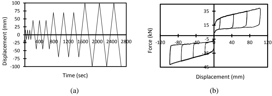
Figure 3. Test results: (a) Applied load-schedule (b) Load-deformation behaviour
