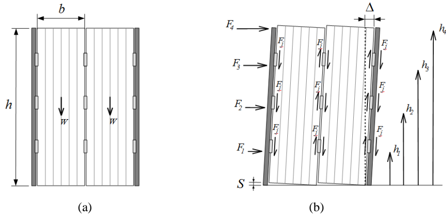
Figure 4. Rocking CLT walls coupled with RSF joints: (a) Before rocking (c) After rocking
