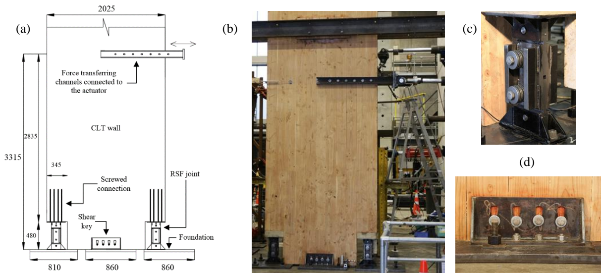
Figure 2. Experimental test of rocking CLT wall with RSF joints: (a) General arrangement (b) Test setup (c) RSF joint (patent no. 7083) (d) Shear key (patent no. 728725)
