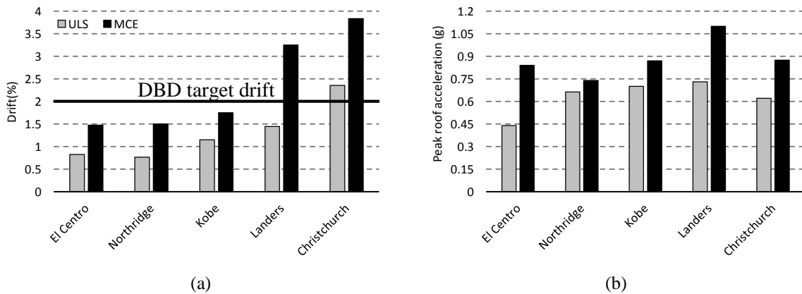
Figure 7. Numerical results: (a) Maximum lateral drifts (b) Peak roof accelerations
