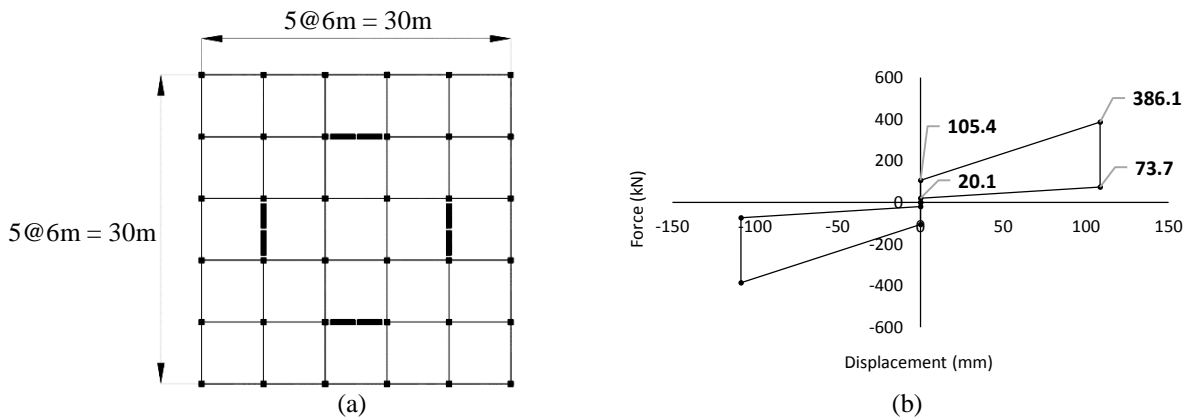
Figure 5. The prototype building: (a) Plan view (b) RSF ductile link design
