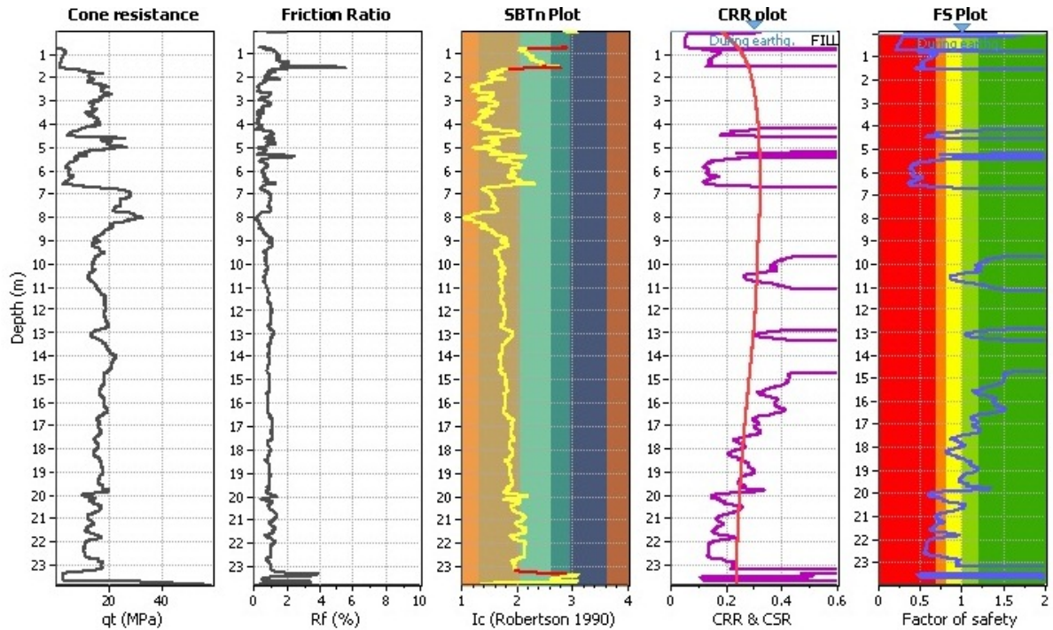
Figure 4. Liquefaction potential analysis based on Roberston and Wride (1998) for the site located in Broomfield Terrace, Christchurch, (GeoLogismiki, 2006).
