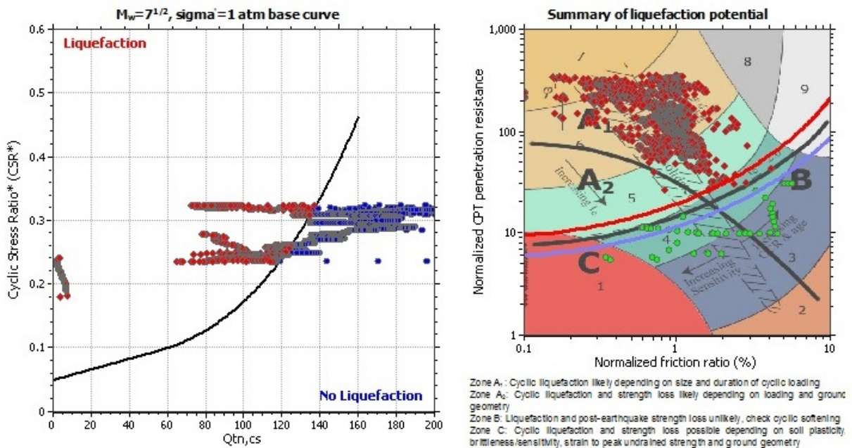
Figure 5. Summary of liquefaction potential analysis based on Roberston (1998) for the site located in Broomfield Terrace, Christchurch, (GeoLogismiki, 2006).
