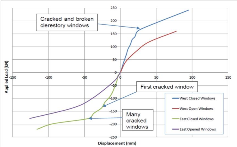
Figure 5. Load-displacement backbone plots for windows closed and windows open
