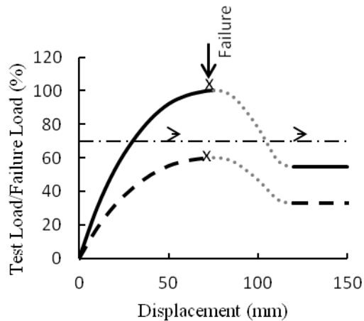
Figure 4: Load-Displacement. Axial tension. Anchor in Wellington greywacke (based on test data from Tonkin & Taylor Ltd files)
