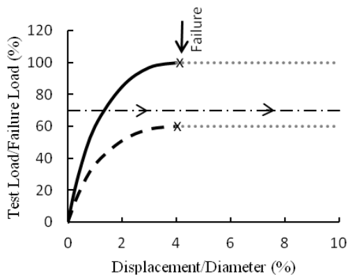
Figure 3: Load-Displacement. Axial compression. Pile in cohesive soil (nominal resistance based on Chen and Kulhawy, 2002)
