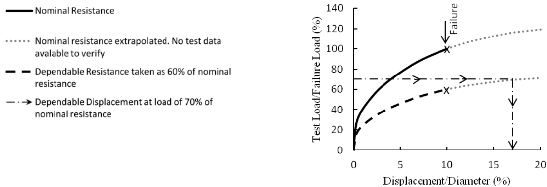
Figure 2: Load-Displacement. Axial compression. Pile in cohesionless soil (nominal resistance based Chen and Kulhawy, 2002)
