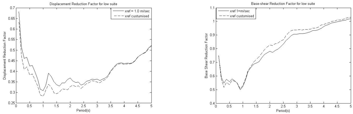
Figure 8: Displacement and base-shear reduction factors for low suite, with \dot{x}_{ref} = 1 \text{ m/s} and \dot{x}_{ref} customised.
