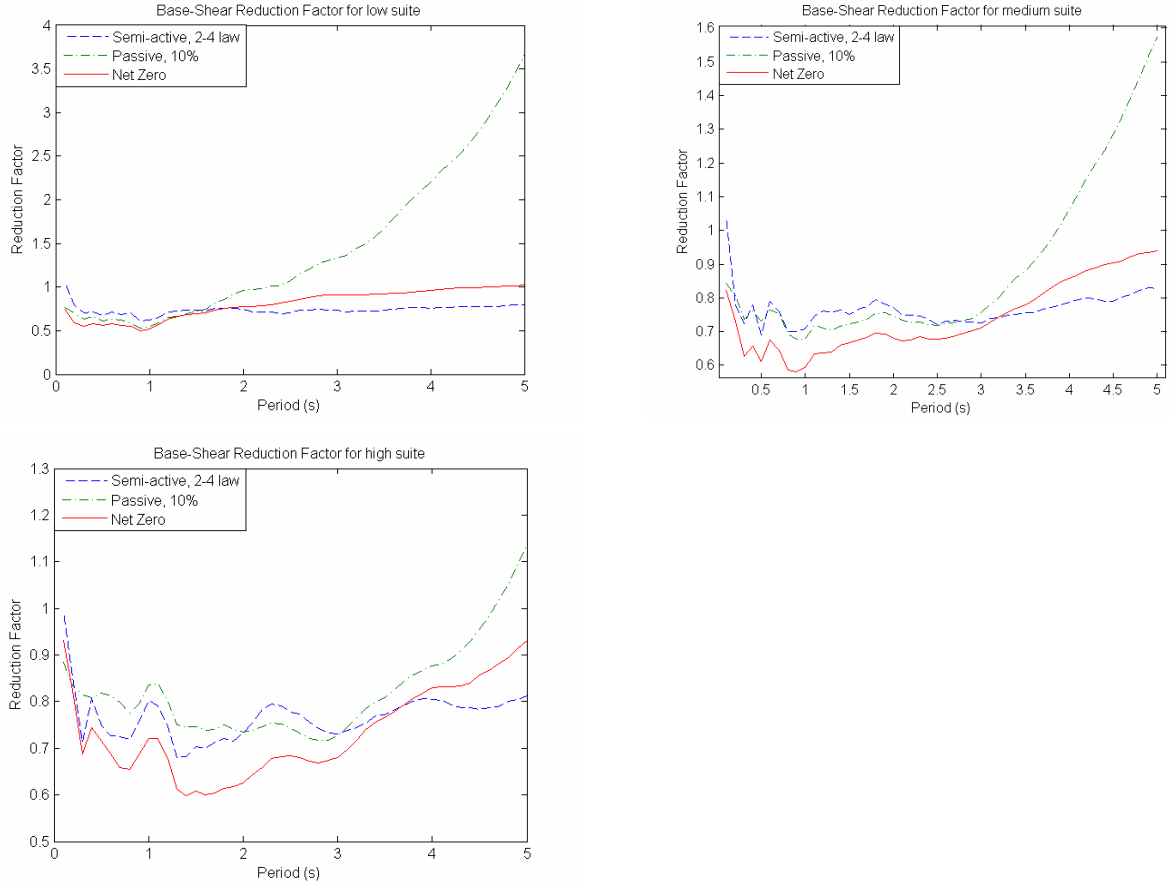
Figure 6: Base-shear reduction factor for low, medium and high suites, using semi-active, passive and net zero damping systems.
