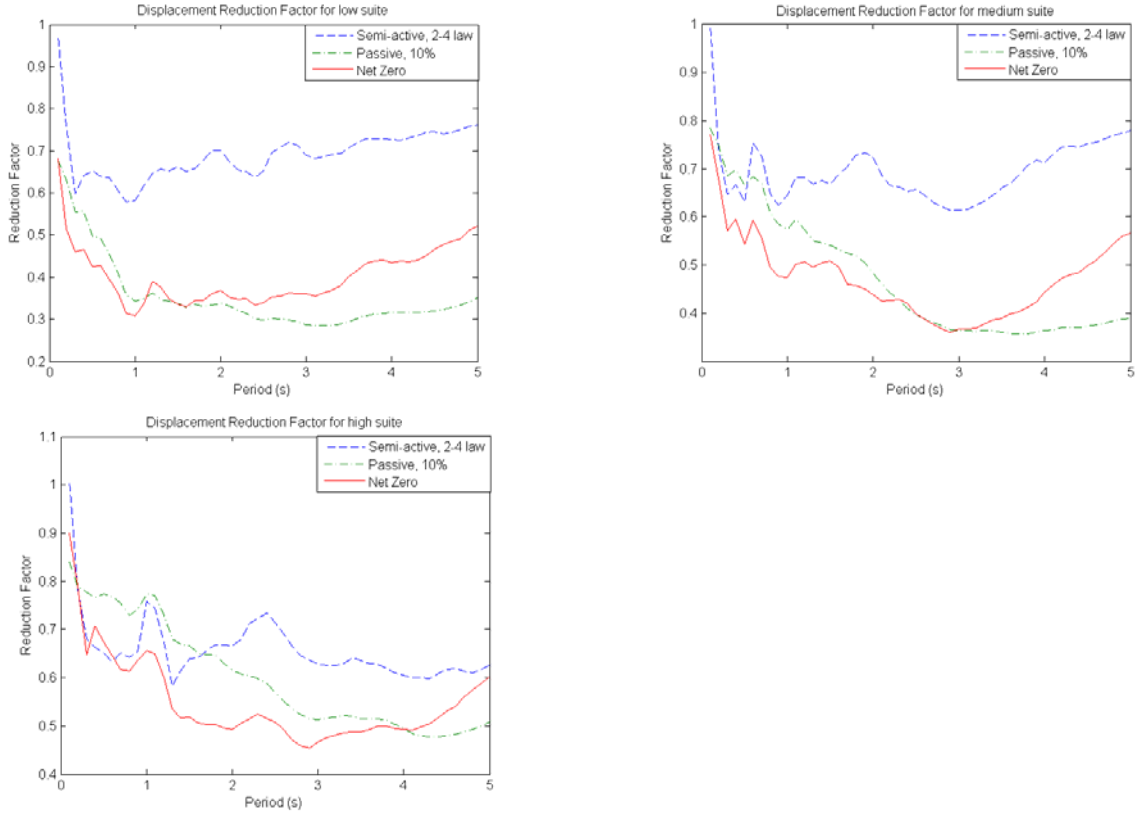
Figure 5: Displacement reduction factor for low, medium and high suites, using semi-active, passive and net zero damping systems.
