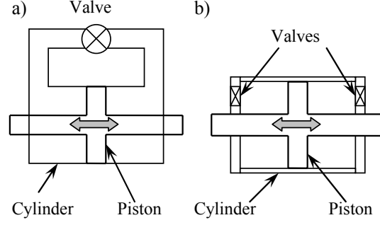
Figure 3: Semi-active device schematics a) Conventional design with single valve and external plumbing system, b) Independent chamber design where each valve vents to atmosphere for a pneumatic device.
