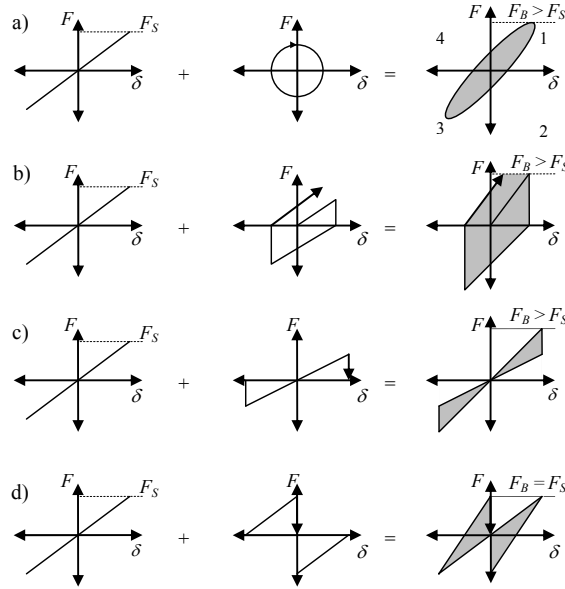
Figure 1: Schematic hysteresis for a) viscous damping, b) a 1-4 device, c) a 2-4 device. F_B = total base shear, F_S = base shear for a linear, undamped structure. F_B > F_S indicates an increase due to the additional damping.
