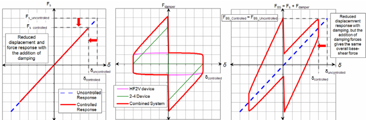
Figure 2: Schematic of the net-zero base-shear concept.
