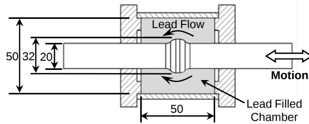
Figure 4: Cross-sectional view of a typical HF2V damper.
