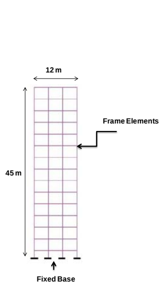
Figure 2. Fixed-base model
