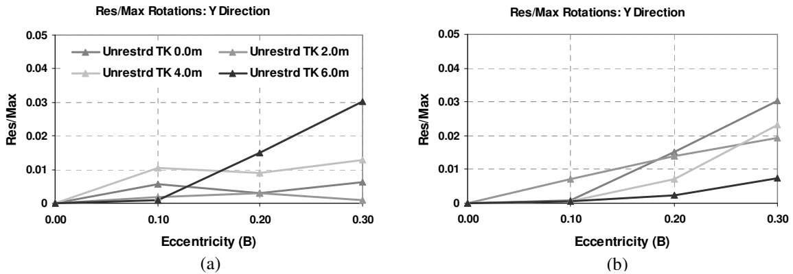
Figure 4. Results indicating the effect of variations in radii of gyration of strength (a) Modified Takeda Unrestrained frame r_{vx} (b) Modified Takeda Restrained frame r_{vz} . (No P- \Delta effects included in analyses)
