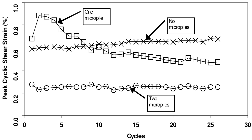
Figure 9. Average peak cyclic shear strain: PGA = 0.40 g, initial Dr = 0.4.
