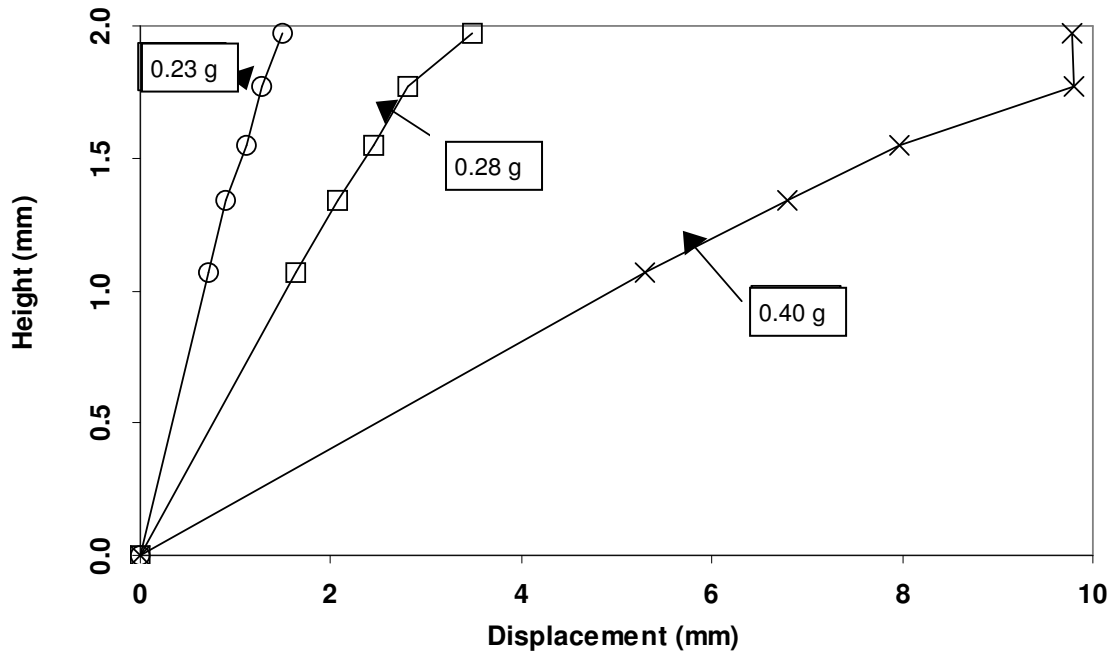
Figure 3. Displacement profiles for unreinforced soil deposits.
