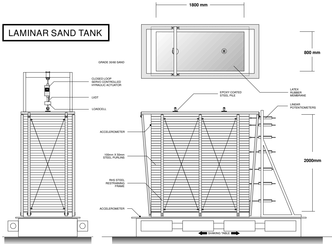
Figure 1. Laminar sand tank
