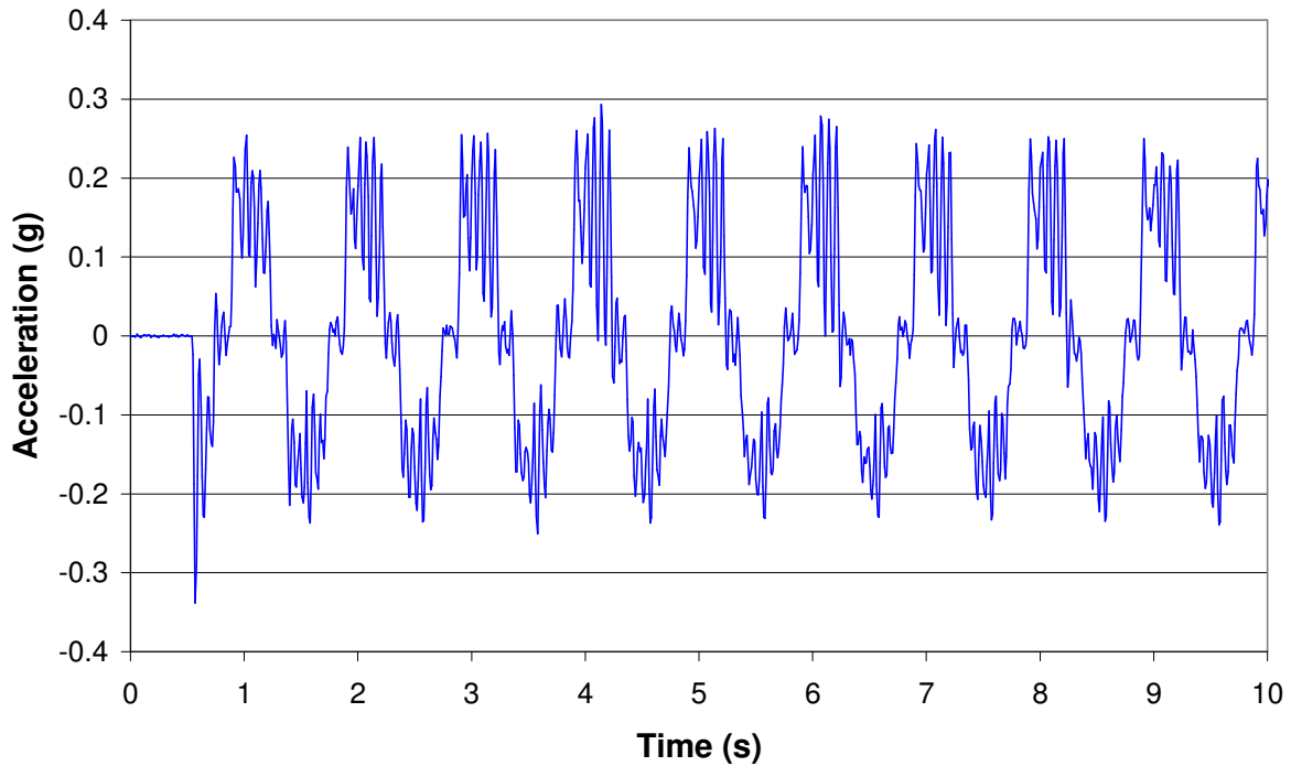
Figure 2. Acceleration Response of Shake Table for +/- 40 mm, 1 Hz shaking.
