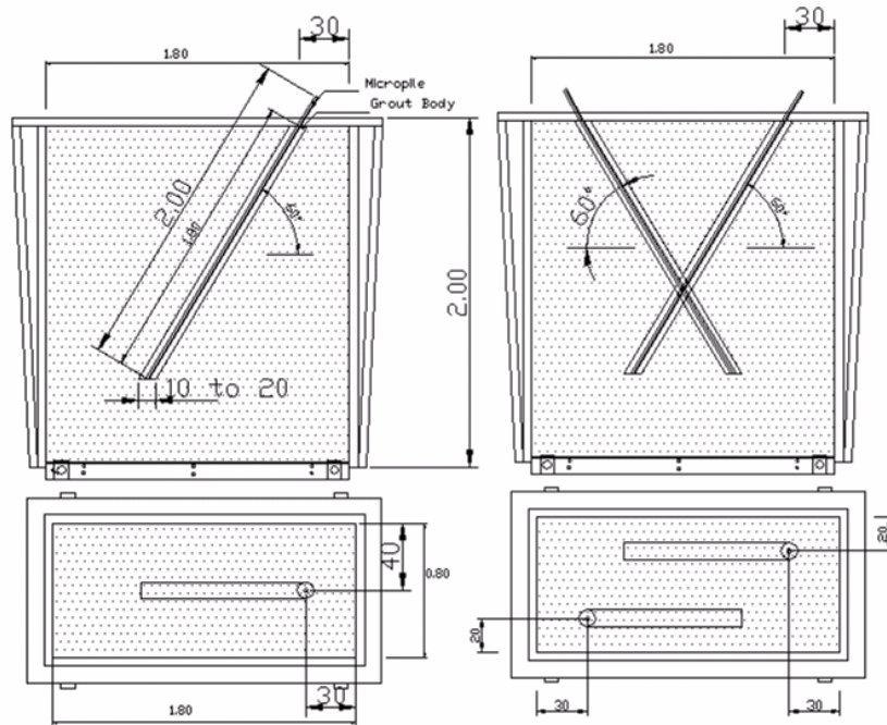
Figure 6. Layout of micropile reinforcement in laminar tank.
