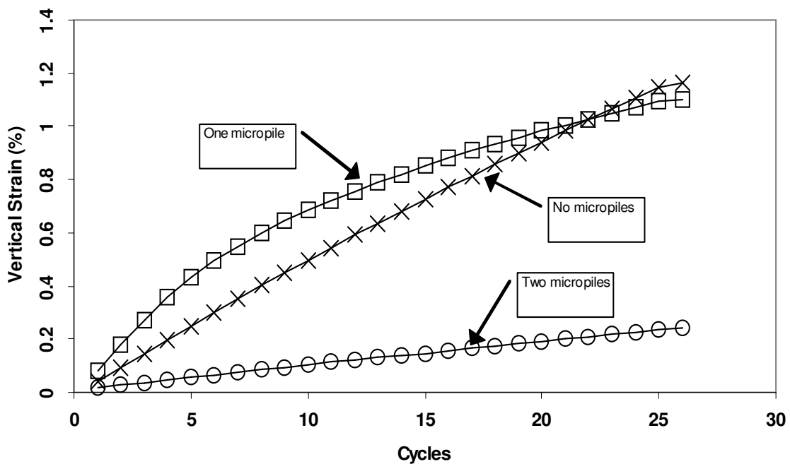
Figure 10. Settlement during shaking: PGA = 0.40 g, initial Dr = 0.4
