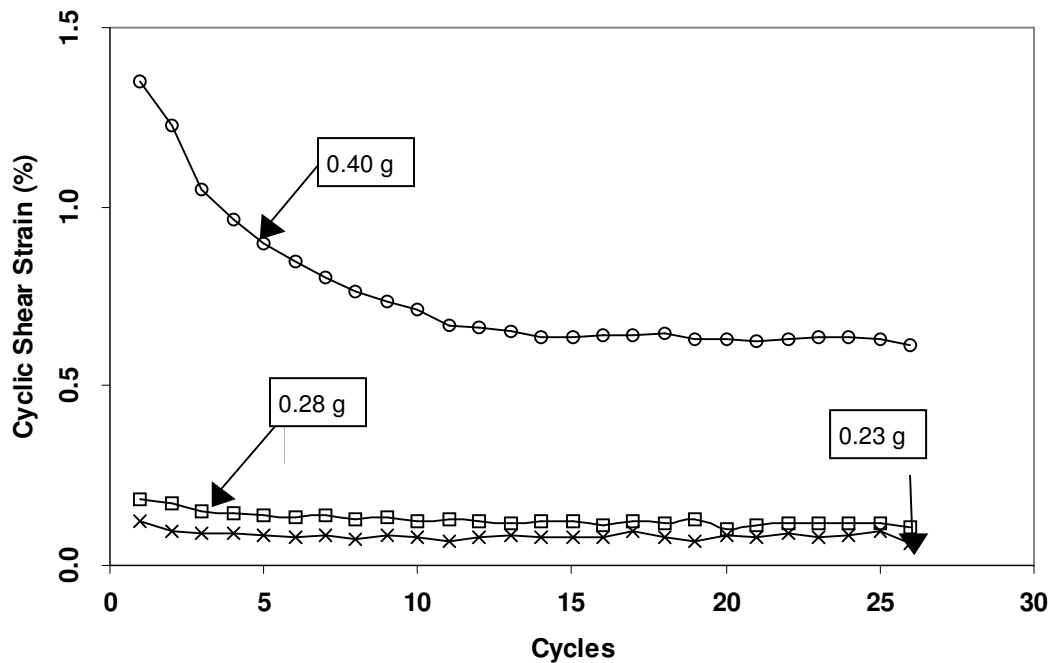
Figure 4. Average peak cyclic shear strain for unreinforced soil deposits (Initial D_r = 0.2 )
