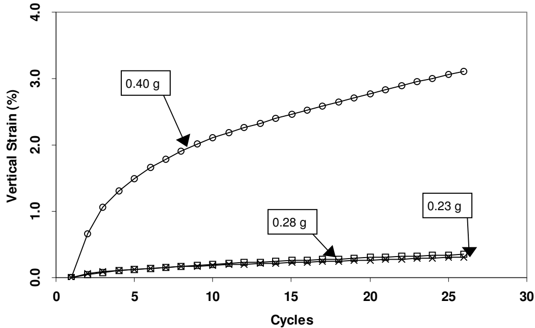
Figure 5. Settlement of unreinforced soil deposits (Initial D_r = 0.2 ).
