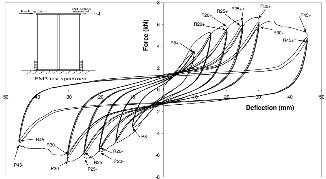
Figure 2. Hysteresis loops from an EM3 test
