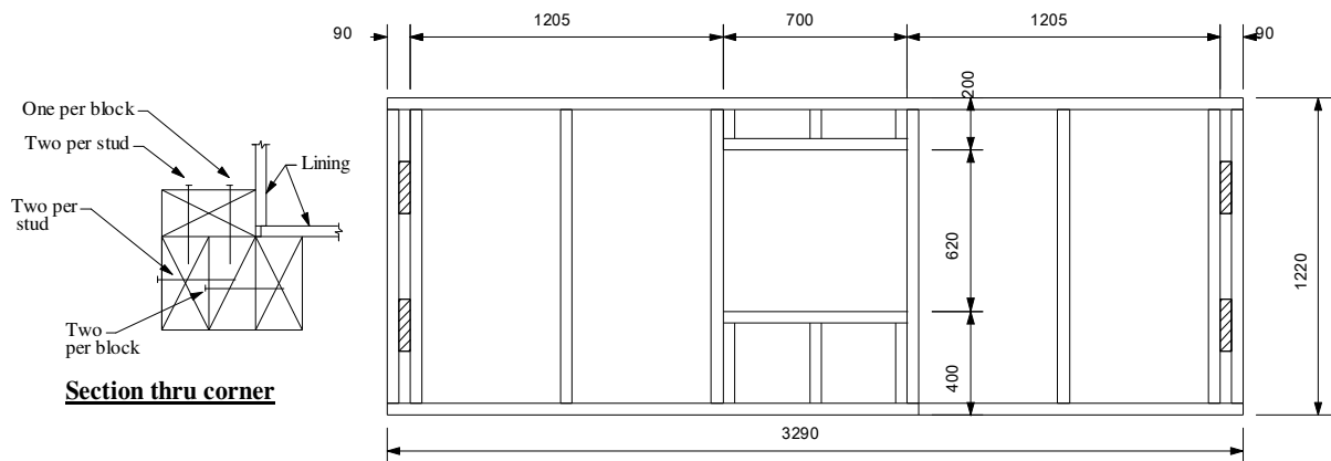
Figure 6. Room racking test – timber framing side walls
