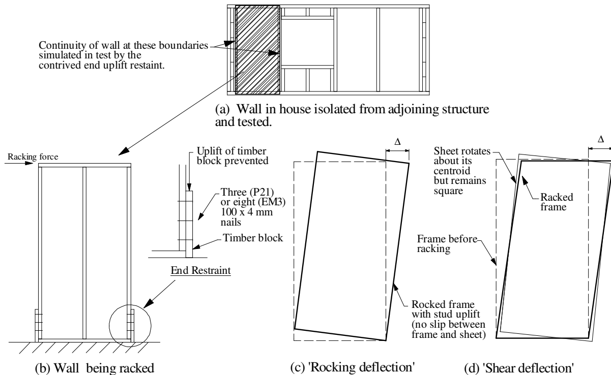
Figure 1: Illustration of a racking test
